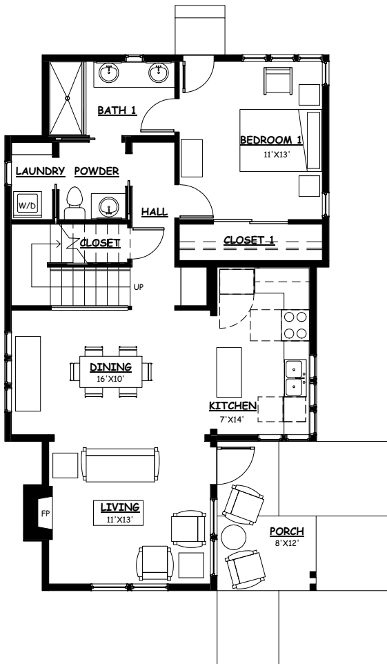
Lower Level 947 sf
